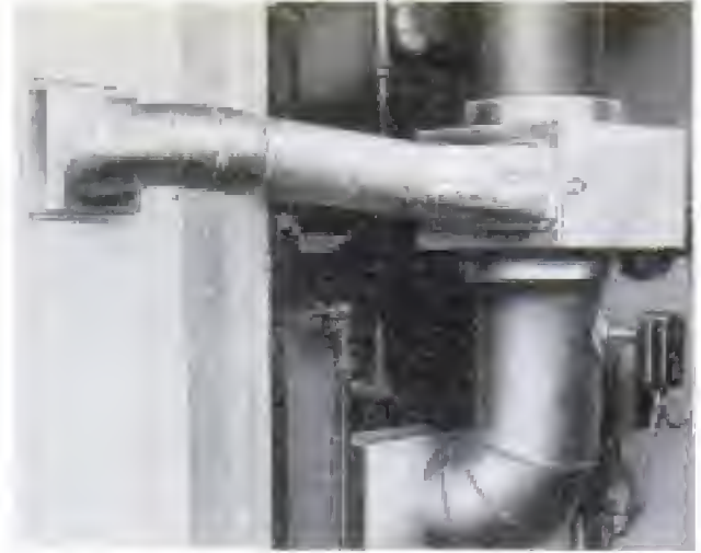
Adapter kit permits use of standard furnace ducts to run heat from exchanger to other parts of house
